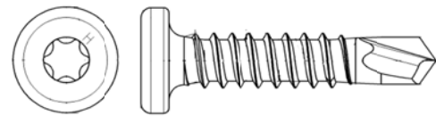
FIGURE 10—TORX PANCAKE HEAD (TPCH) SD FRAMER SELF-DRILLING SCREW
