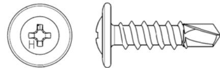
FIGURE 8—PHILLIPS TRUSS HEAD (PTH) SD FRAMER SELF-DRILLING SCREW
