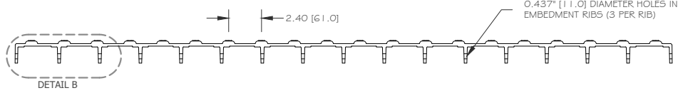
CC SECTION
