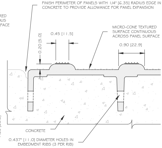
B DETAIL - INSTALLED IN CONCRETE
