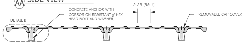
CC SECTION
