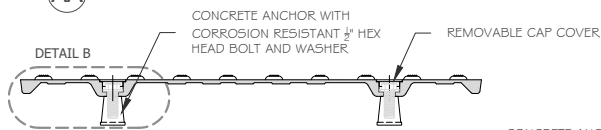
CC SECTION
