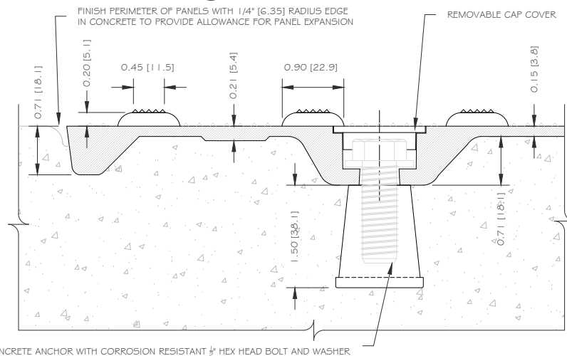
B DETAIL - INSTALLED IN CONCRETE
