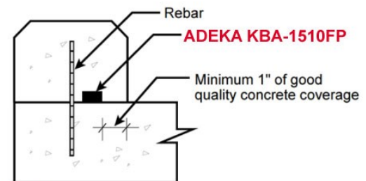
Containment curb
