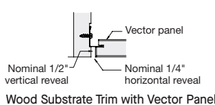
Wood Substrate Trim with Vector Panel
