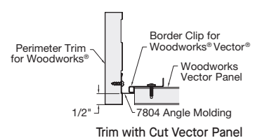
Trim with Cut Vector Panel
