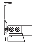
Aluminum Substrate Trim Assembly for Vector Panel
