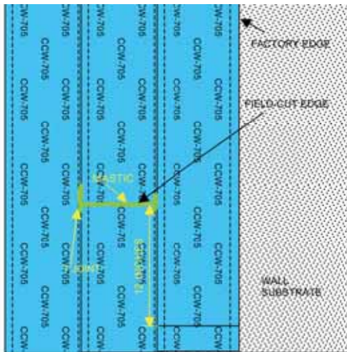
Figure 2: Installation in Vertical Runs
