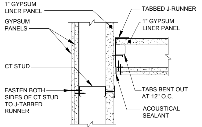
11 WALL JUNCTION
