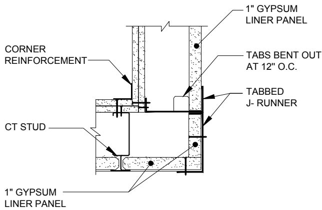
10 INSIDE CORNER
