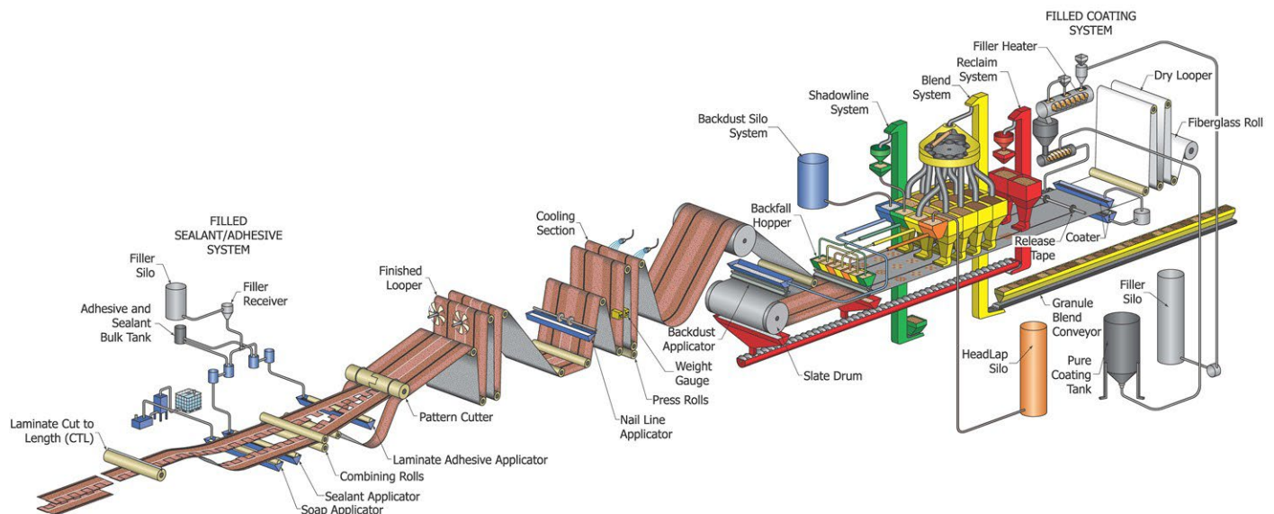
Figure 2: Laminated shingle production diagram
