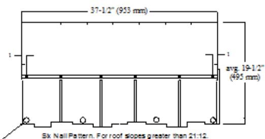
FIGURE 1—SHINGLE PROFILES AND FASTENER PATTERNS (Continued)
