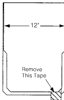
Figure 17-18: Shingle Ridge®.
