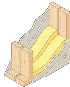
Figure 13: Double stud construction permits twice the thickness of fiberglass sound absorbing insulation. STC rating of 66-67 is excellent. See page 26.
