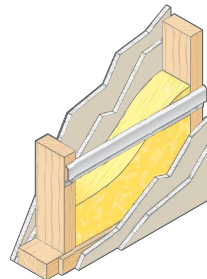
Figure 12: Resilient channels help minimize transmission of vibration through wall. STC rating of 57-59 considered acceptable for most uses. See page 24.
