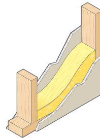
Figure 10: Conventional wood stud construction, single layer gypsum wallboard each side, 3-1/2" thick fiberglass insulation in wall cavity. STC: 39.
