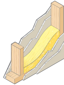
Figure 11: Conventional wood stud construction, double layer gypsum wallboard each side. Increased mass boosts STC rating to 55. See page 23.
