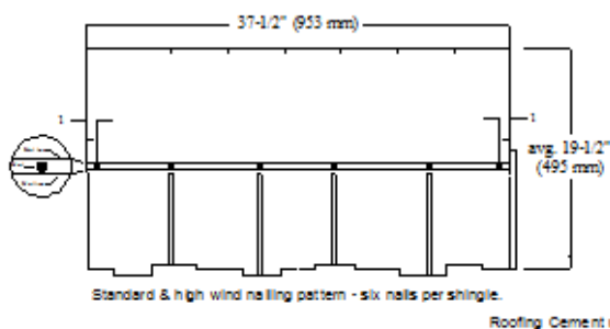
FIGURE 1—SHINGLE PROFILES AND FASTENER PATTERNS (Continued)
