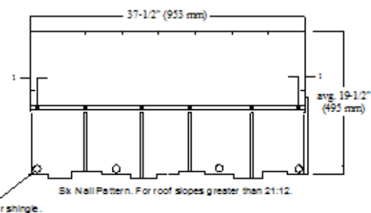
FIGURE 1—SHINGLE PROFILES AND FASTENER PATTERNS (Continued)
