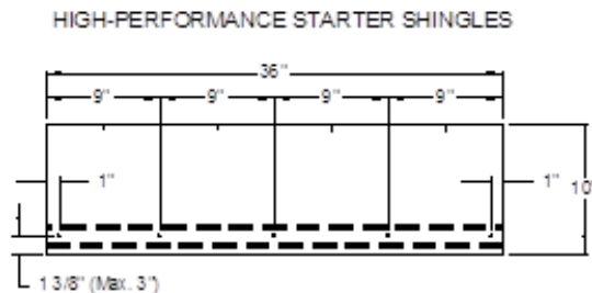
FIGURE 1—SHINGLE PROFILES AND FASTENER PATTERNS (Continued)
