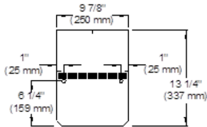
Nailing pattern all applications - two nails per shingle.
