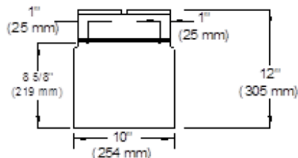
Nailing pattern all applications - two nails per shingle.
