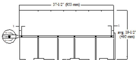
Standard & high wind nailing pattern - six nails per shingle.
