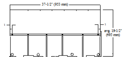
Six Nail Pattern. For roof slopes greater than 21:12.
