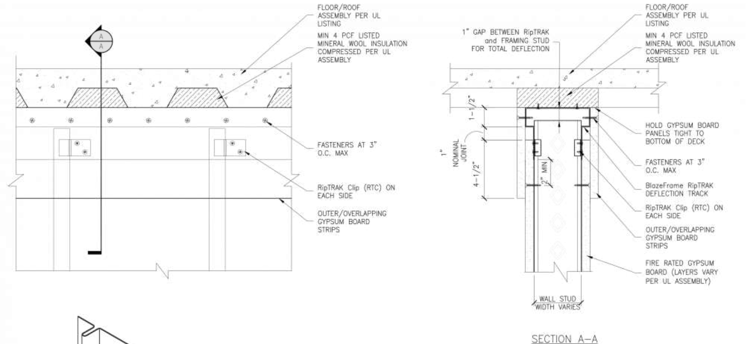
HEAD OF WALL DETAIL RT1-2-UD-2-ALT UL LISTED FLOOR/ROOF ASSEMBLY W/ UNPROTECTED DECK (UD) - MINERAL WOOL FILL
