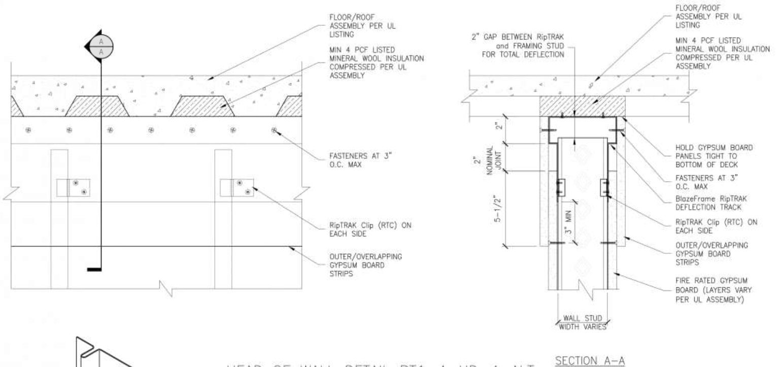
HEAD OF WALL DETAIL RT1-4-UD-4-ALT UL LISTED FLOOR/ROOF ASSEMBLY W/ UNPROTECTED DECK (UD) - MINERAL WOOL FILL
