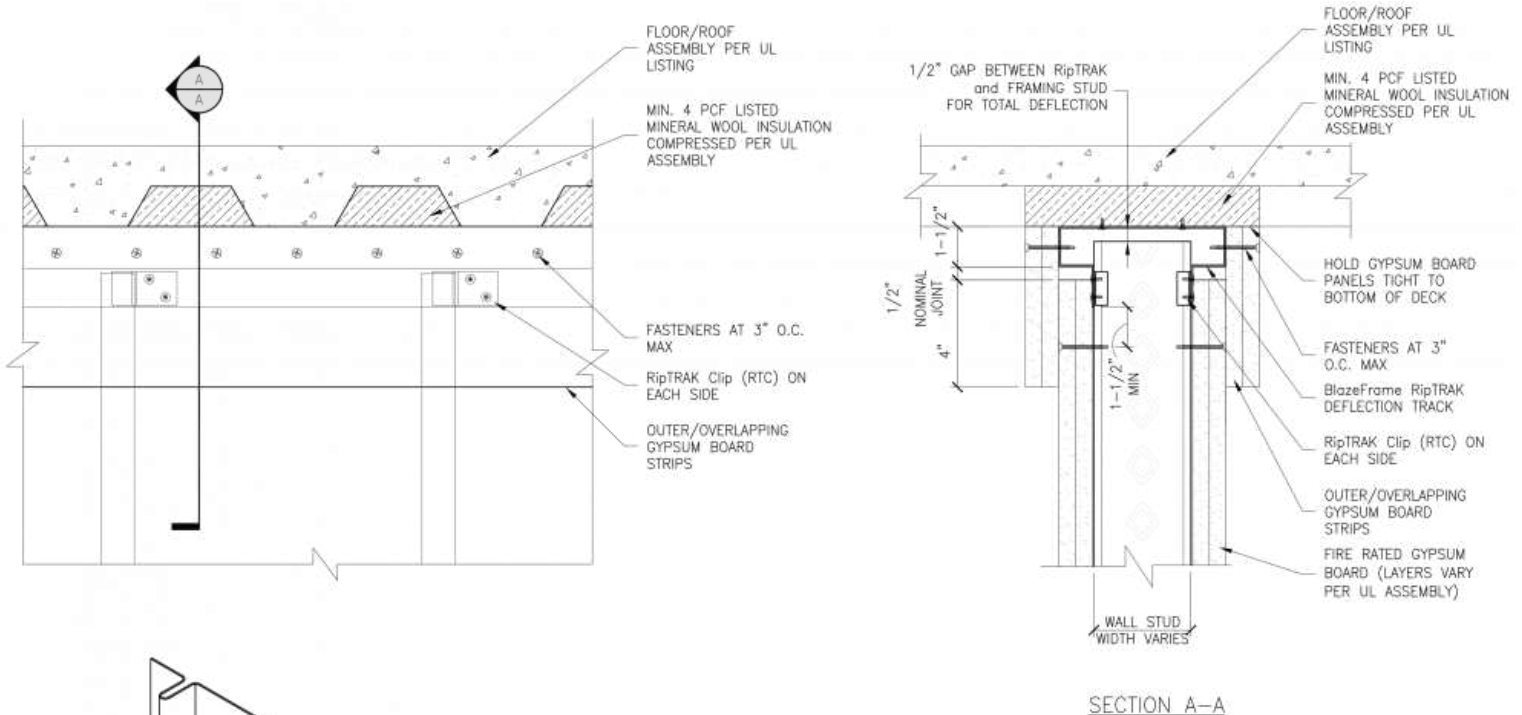
HEAD OF WALL DETAIL RT2-1-UD-1-ALT UL LISTED FLOOR/ROOF ASSEMBLY W/ UNPROTECTED DECK (UD) - MINERAL WOOL FILL
