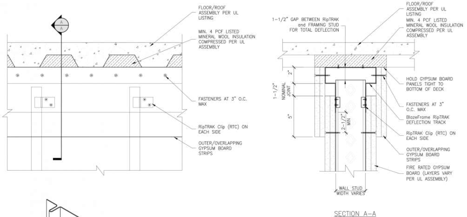
HEAD OF WALL DETAIL RT2-3-UD-3-ALT UL LISTED FLOOR/ROOF ASSEMBLY W/ UNPROTECTED DECK (UD) - MINERAL WOOL FILL
