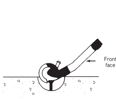
Initial positioning of the P51 Swift Lift Lifting Eye onto the Swift Lift Anchor
