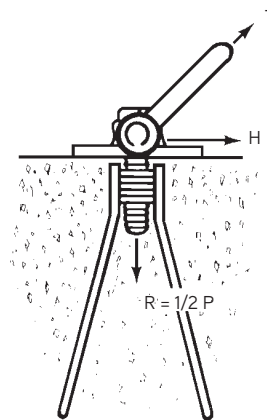
Detail A
