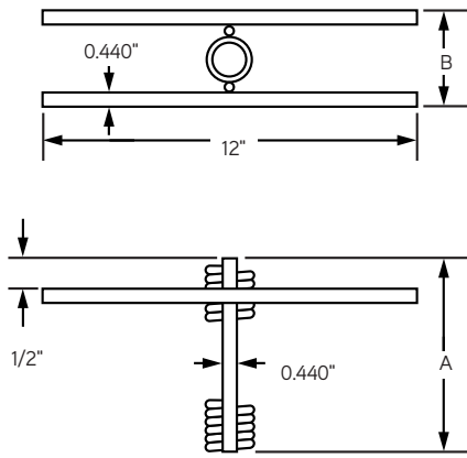
T10 Single End Pickup Insert
