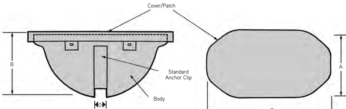
P99D Fleet-Lift Disposable Recess Plug
