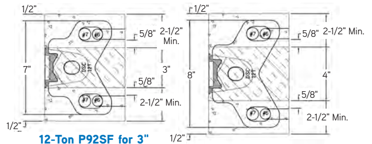
12-Ton P92SF for 3" Insulation 12-Ton P92SF for 4" Insulation
