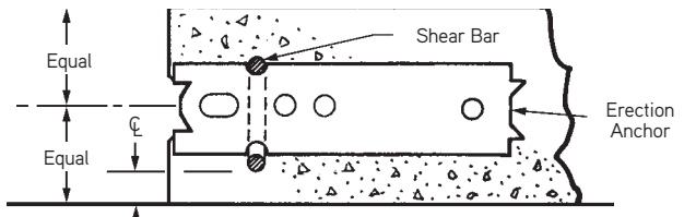
Minimum 3/4" Concrete Cover
