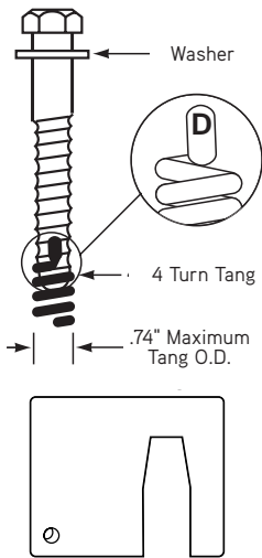
T13 Coil Anchor Bolt Patent #5,006,023 3/4" Dia. x 6" Long
