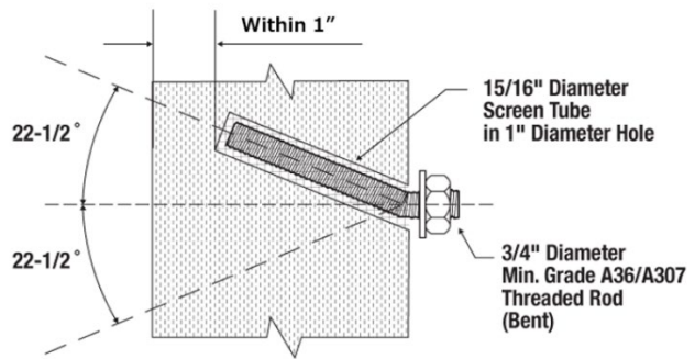
FIGURE 2—CONFIGURATION B (22 1 / 2 -DEGREE COMBINATION ANCHOR) 1
