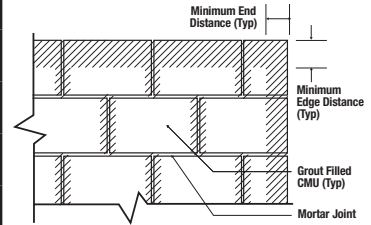
Wall Face Permissible Anchor Locations (Un-hatched Area)
