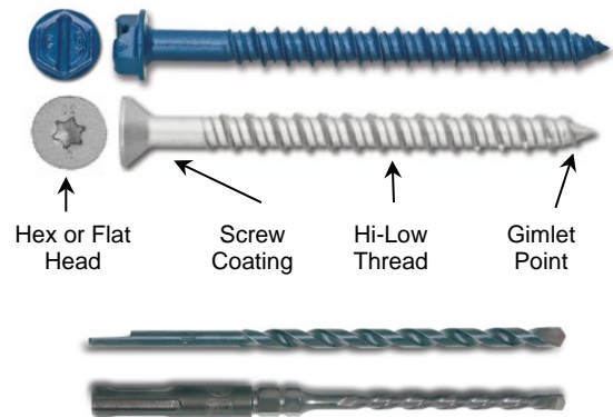
FIGURE 2—ULTRACON+ SCREW ANCHOR AND DRILL BITS (Slotted Hex Head and star drive flat head shown for illustration – Shank and thread specifications are the same for screws with other head types.)
