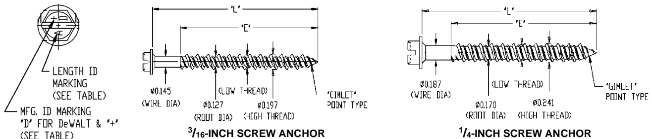
FIGURE 1—FASTENER SPECIFICATIONS FOR ULTRACON+ SCREW ANCHOR
