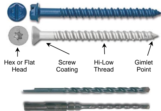
FIGURE 2—ULTRACON+ SCREW ANCHOR AND DRILL BITS
