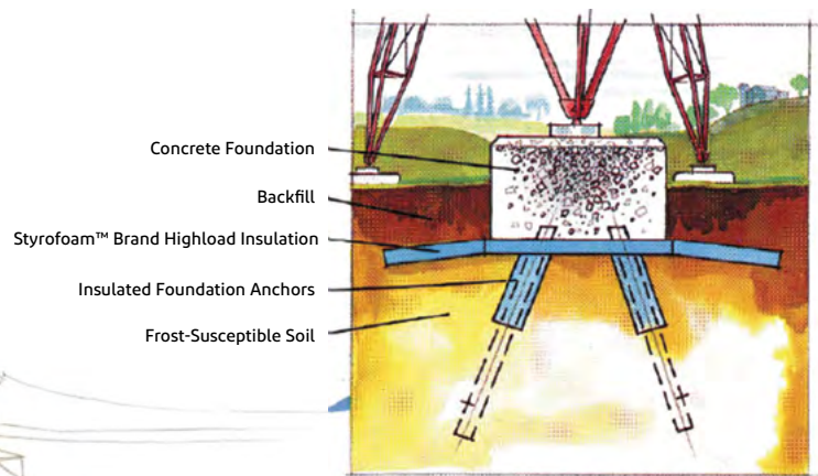
Guyed Tower Foundation
