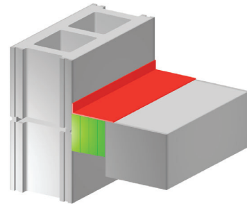
Typical Floor to Wall Joint
