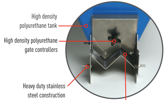
Stainless steel gates accommodate off-angles, inside 90s, bullnose, and outside 90s
