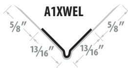
A1XW EL Tape-On Extra Wide Outside Corner
