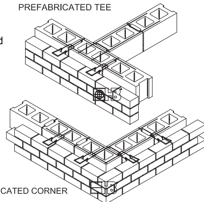
PREFABRICATED TEE
