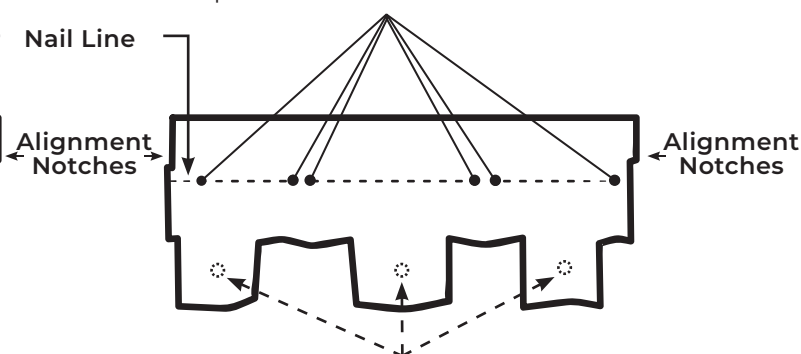
Nailing – Steep Slopes/High Wind Areas Applications Requires 6 Nails
