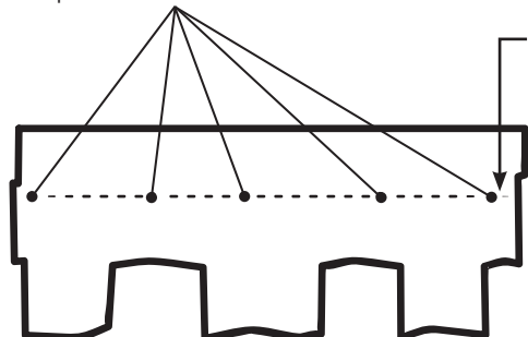
Standard Application Requires 5 Nails
