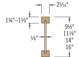
TJI® 230 joists
