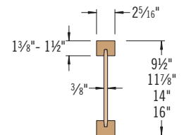
TJI® 360 joists
