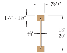
TJI® 360 joists
