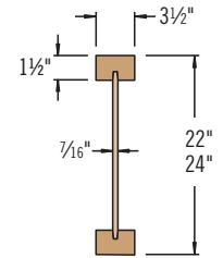
TJI® 560D Joist
