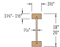
TJI® 560 joists
