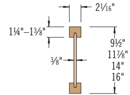
TJI® 210 joists
