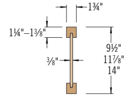
TJI® 110 joists
