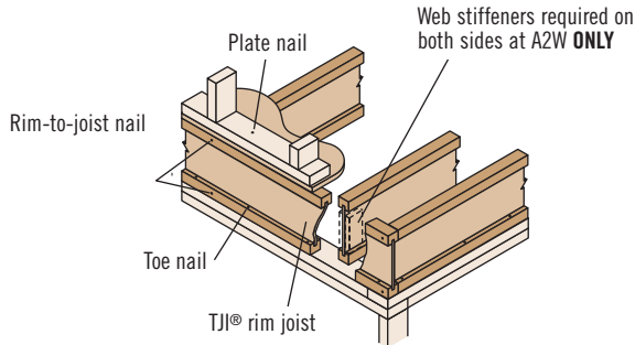
A2 A2 W Must have 1 1/4" minimum joist bearing at ends. Attach rim joist per fastening instructions in Detail A3.
