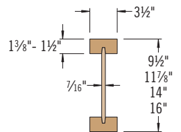
TJI® 560 joists
