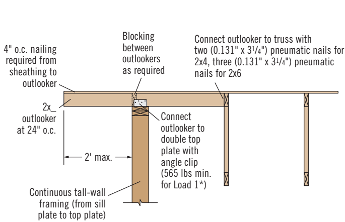
WB2 * Load 1 value from Lateral Connections—Angle Clips table below.
