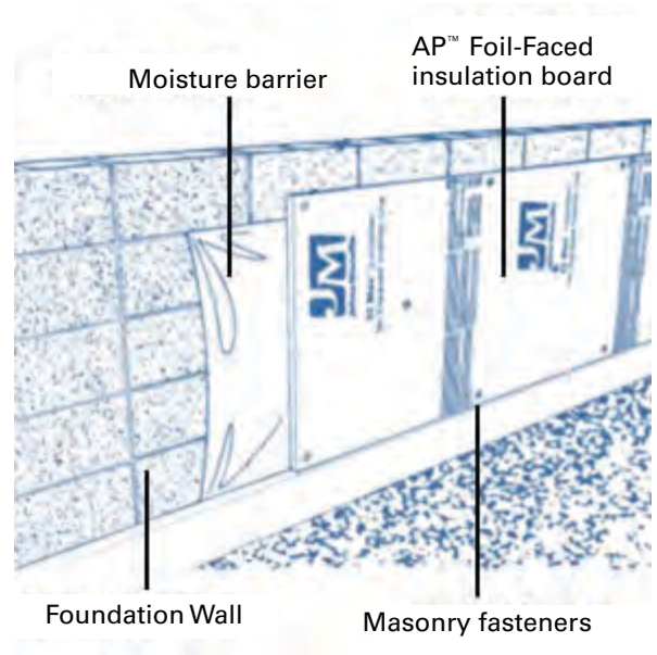
Figure 2. Unvented Crawl Space
