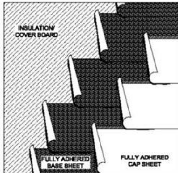
Figure 3: APP modified bitumen roof membrane system installation details
