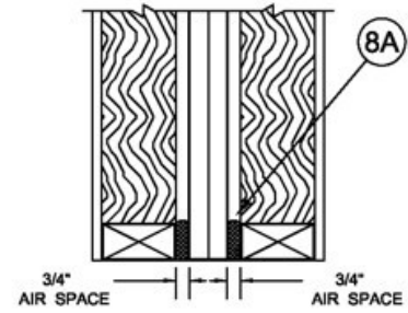
SECTION B1-B1
