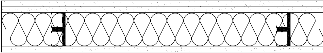
3-5/8" WALL WITH 2X1 APPLICATION
