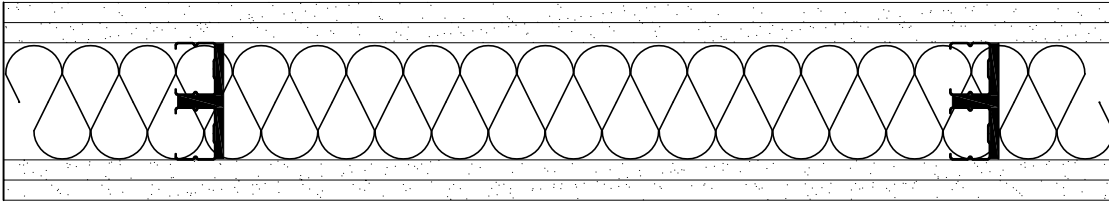
3-5/8" WALL WITH 2X2 APPLICATION
