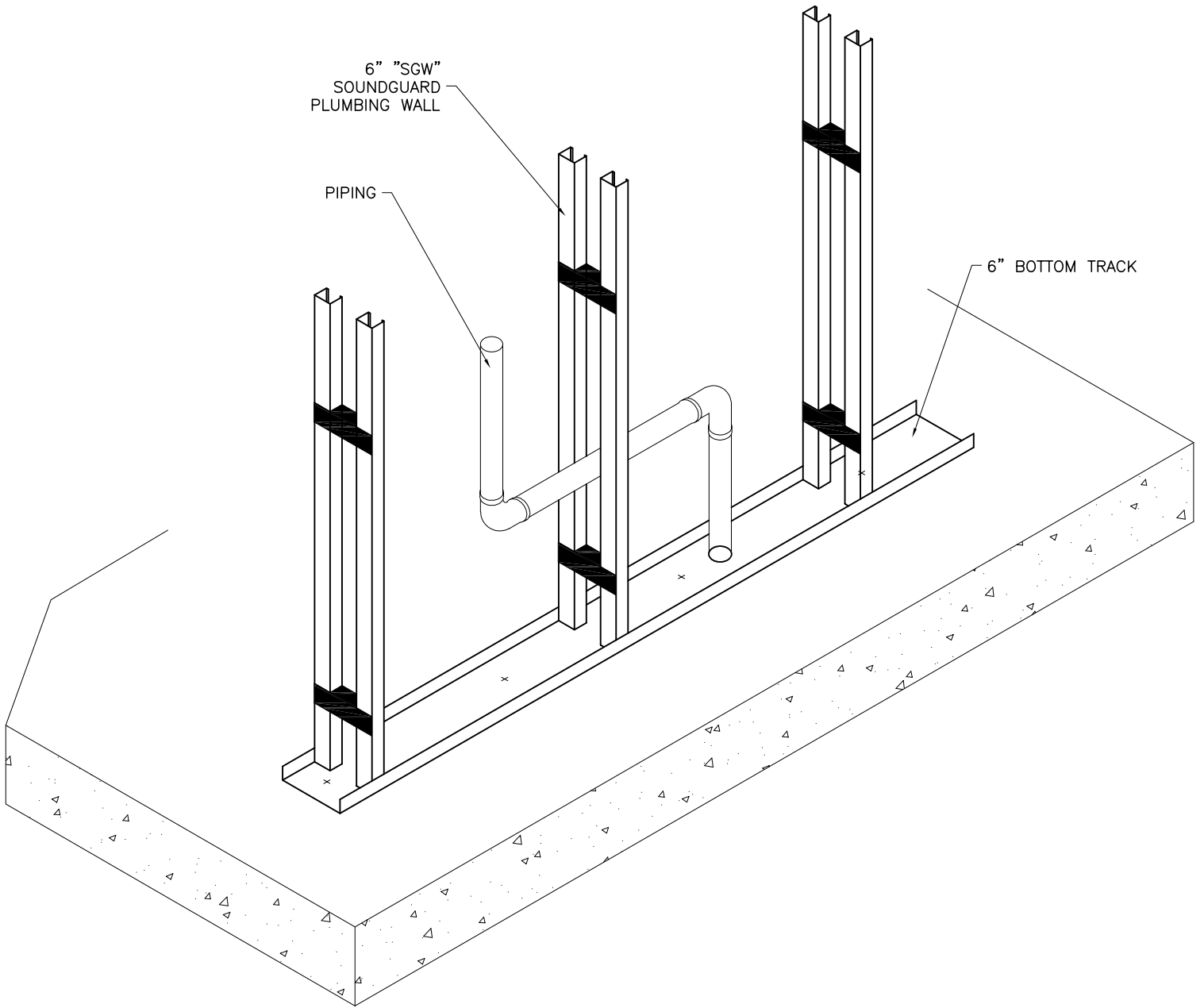
10 SOUNDGUARD PLUMBING WALL DETAIL
