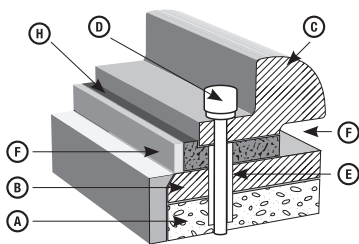
Figure 5 - Typical Epoxy Chock Application
