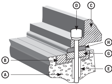
Figure 3 - Rail or Soleplate
