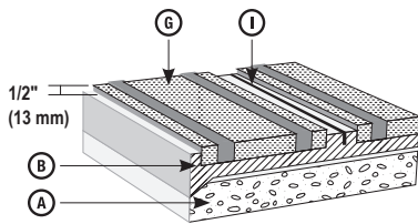
Figure 4 - Typical Rail With Expansion Joint Section
