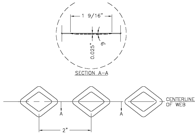
FIGURE 2 – WEB EMBOSSMENT DETAIL (No embossment on 1-5/8" studs)
