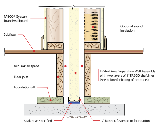
TYPICAL FOUNDATION DETAIL Elevation View
