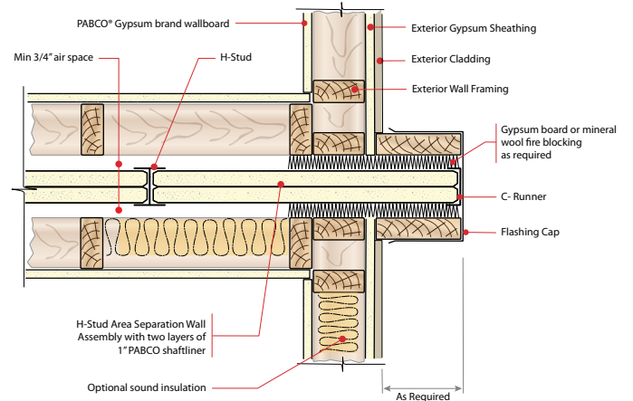
PROTRUDING EXTERIOR WALL INTERSECTION DETAIL Plan View
