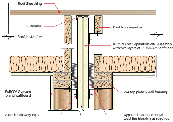
TYPICAL ROOF INTERSECTION DETAIL Elevation View
