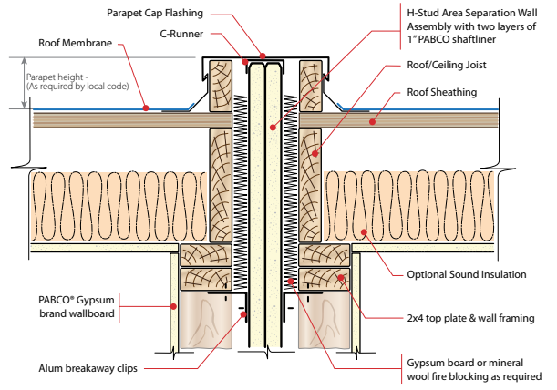
TYPICAL ROOF INTERSECTION PARAPET DETAIL Elevation View
