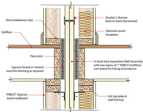
TYPICAL INTERMEDIATE FLOOR DETAIL Elevation View
