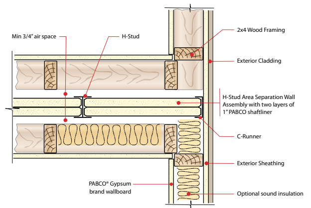
EXTERIOR WALL INTERSECTION DETAIL Plan View
