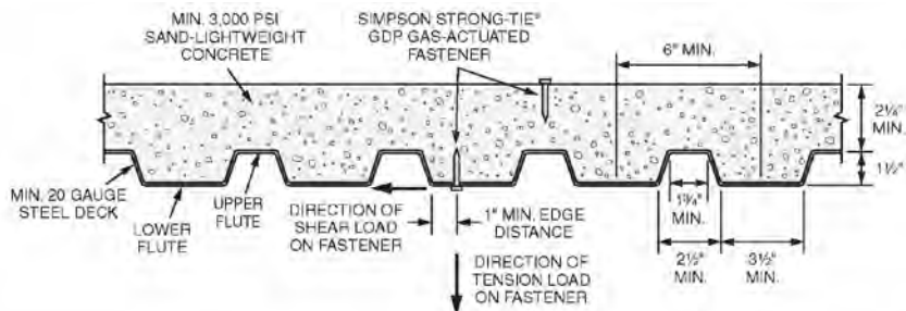
FIGURE 1B—GDP GAS-ACTUATED FASTENER INSTALLED INTO CONCRETE FILLED INVERTED 1/2-INCH-DEEP COMPOSITE FLOOR “B” DECK
