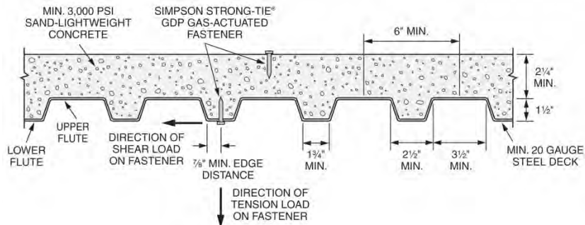
FIGURE 1A—GDP GAS-ACTUATED FASTENER AND GRH AND GAC ASSEMBLIES INSTALLED INTO CONCRETE FILLED 1/2-INCH-DEEP COMPOSITE FLOOR “B” DECK
