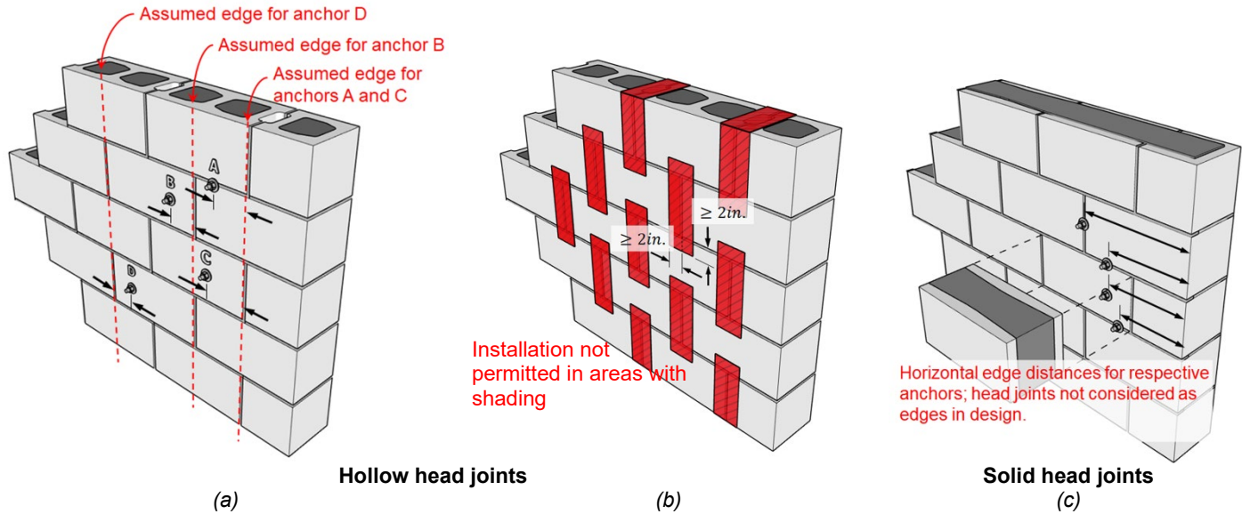
FIGURE 1—(a) Edge distance considerations in fully grouted CMU construction with hollow head joints, (b) exclusion zones in fully grouted construction with hollow head joints, and (c) edge distance considerations in fully grouted CMU construction with solid head joints . Note: dimensions to upper and lower edges omitted for clarity.
