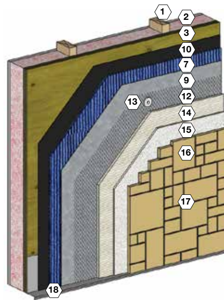
EXTERIOR-CEMENT BOARD
