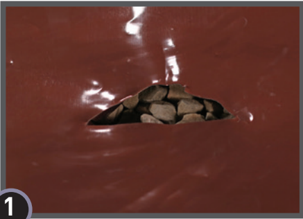
1 Occasionally there are larger holes in the vapor barrier that require a patch.
