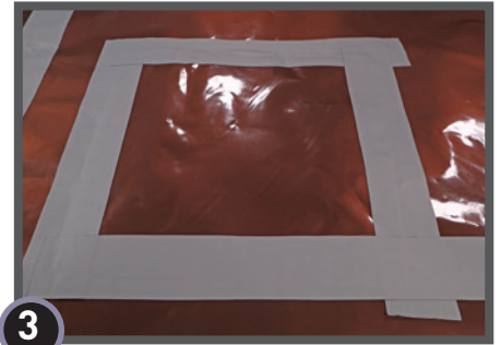
3 Seal the patch with DragoSeal Tape.
