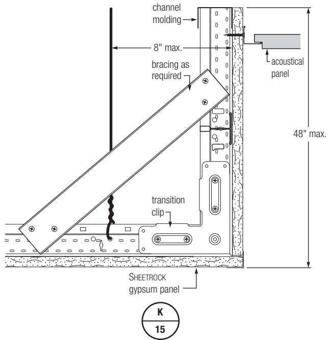
Section through soffit and acoustical transition
