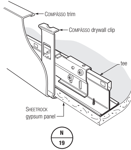
Compasso Trim parallel to main tee or cross tee
