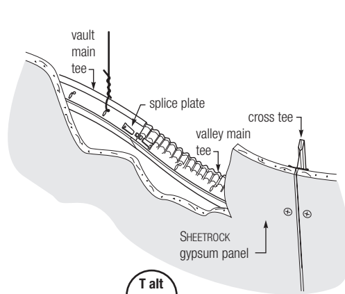
Vault to valley—factory-end connection
