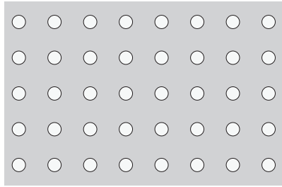
6mm hole on 16mm spacing 10% open area
