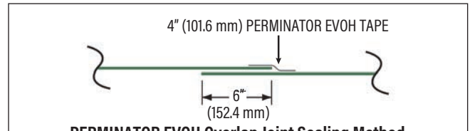
PERMINATOR EVOH Overlap Joint Sealing Method Vapor Retarder Applications
